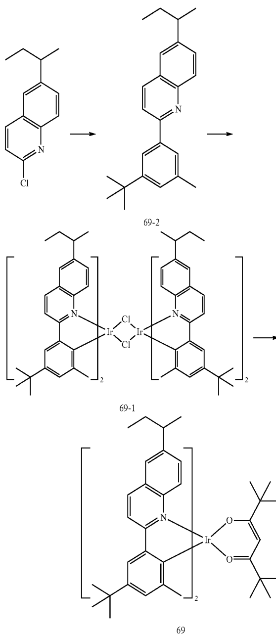
Reaction Scheme 6
