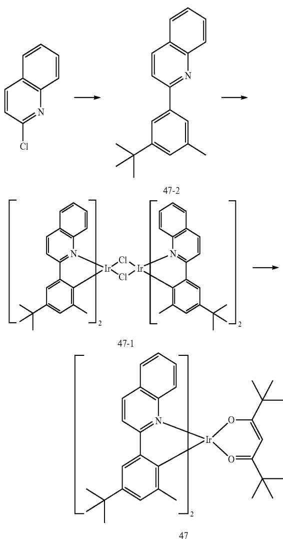
Reaction Scheme 5
