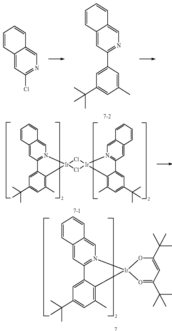
Reaction Scheme 2
